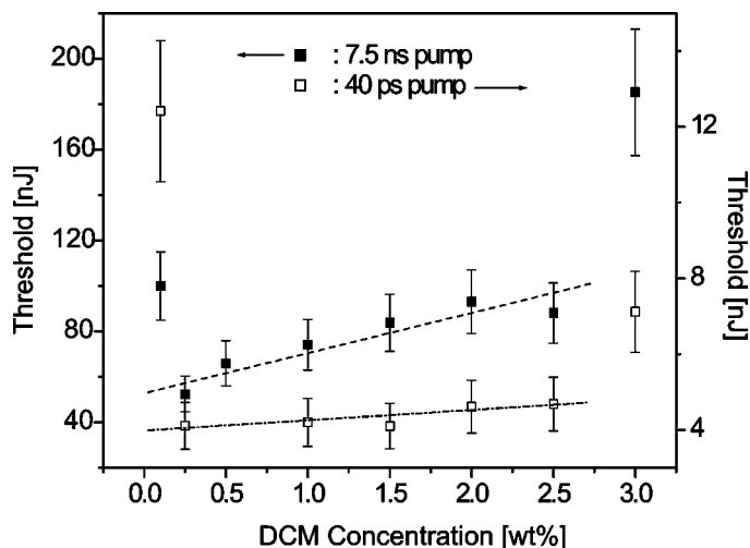
FIGURE 2 Dependence of lasing threshold on dye concentration with nano-second and picosecond pump pulses. The dotted lines are linear fits in the concentration region of 0.25 wt% to 2.5 wt%.
