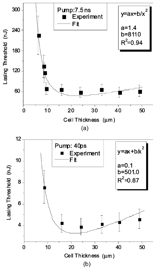
FIGURE 6 Lasing threshold as function of sample thickness. (a) nanosecond pump (b) picosecond pump.
