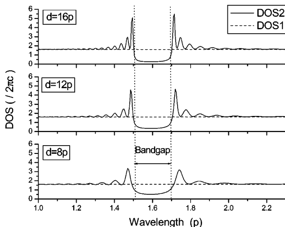
FIGURE 7 Calculated DOS for the two normal modes as a function of cell thickness. The dotted lines are the reflection band edges of a semi-infinite sample, n_o = 1.51 , n_e = 1.70 .
