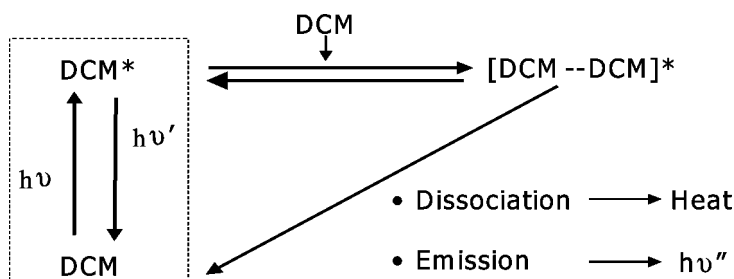
FIGURE 4 Excimer formation and decay. DCM*: excited DCM molecule, [DCM-DCM]*: DCM excimer. The dotted frame shows the process when dye concentration is low.
