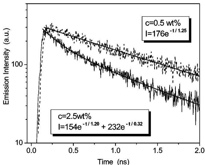
FIGURE 5 Fluorescence decay at 608 nm with DCM concentrations of 0.5 wt% and 2.5 wt%. The pump pulsewidth is 40 ps.
