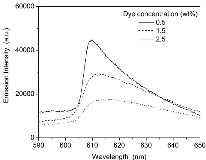
FIGURE 3 Fluorescence quenching: fluorescent emission for different dye concentrations. The pump pulsewidth is 7.5 ns.
