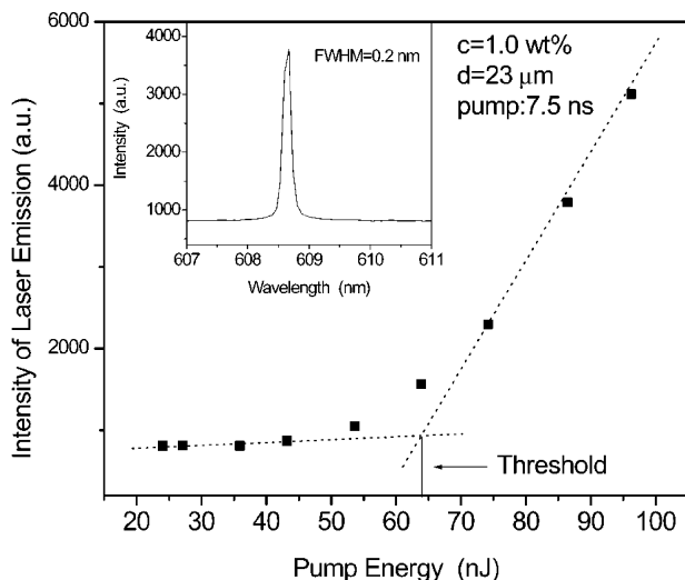
FIGURE 1 Intensity of CLC laser emission as function of pump energy.
